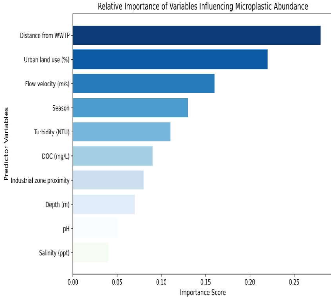
Fig 3 : Relative importance of environmental and anthropogenic predictors controlling microplastic abundance. Distance from WWTP and urban land use exert the strongest influence, followed by hydrodynamic and seasonal controls.
