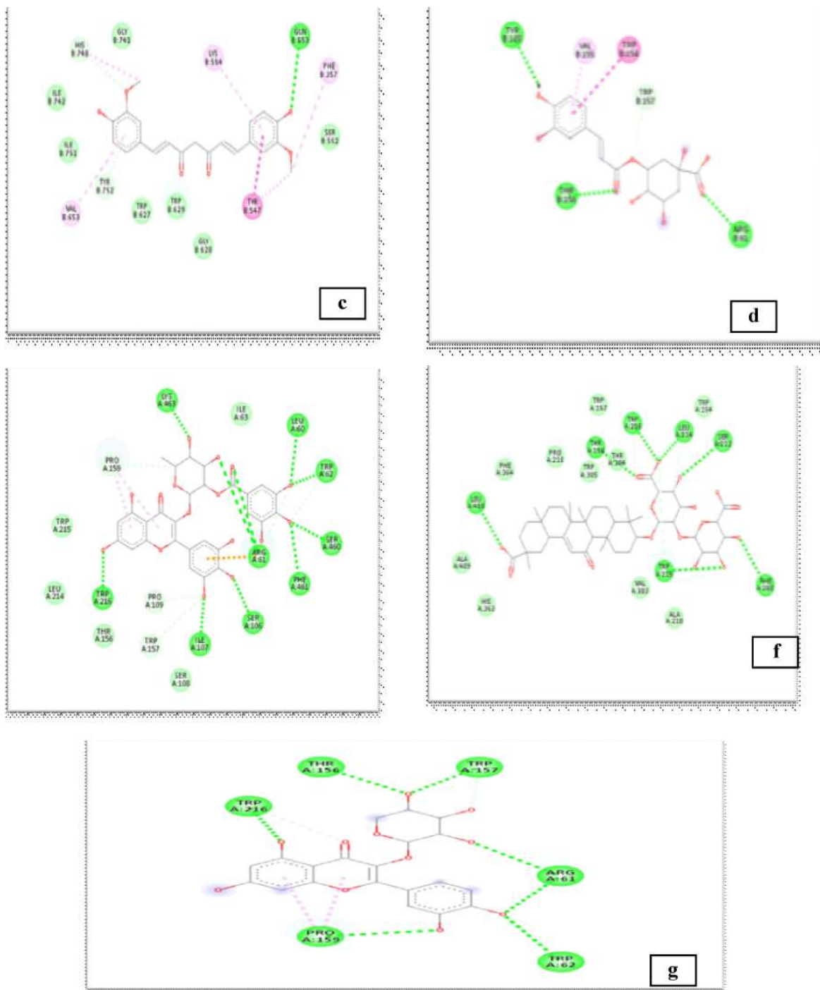
Figure 2: Images of docking interaction of herbal molecules with 1PFQ (dipeptidyl peptidase4) ligands (a) AsparasaponinII (b) Baohuside1 (c) curcumin (d) Chlorogenic Acid (e) Desmanthin1 (f) Guaijaverin (g) Glycyrrhizin.
