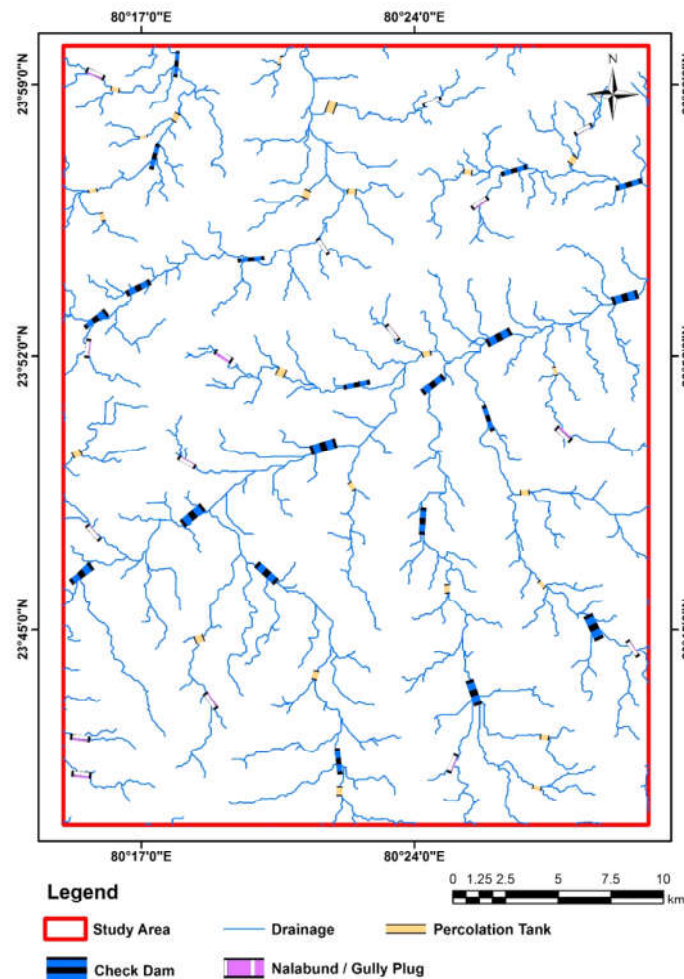
Figure 2 : Water conservation structures in the study Area
