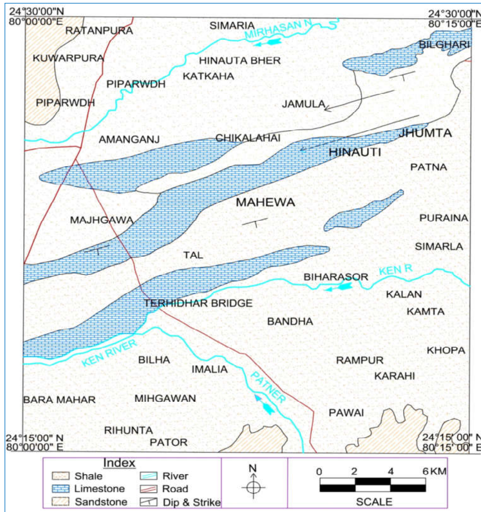
Fig 1 Geological Map of the Study Area
