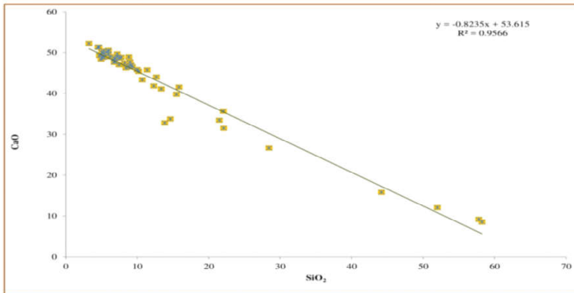
Fig. 5 : The figure shows direct inverse correlation between CaO and SiO 2 , Jhumta Area
