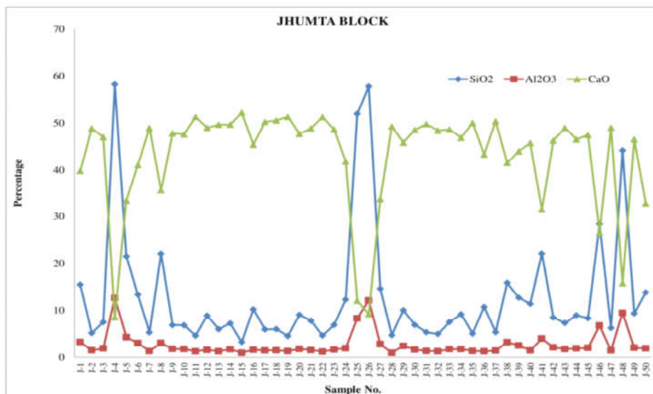
Fig. 4 : SiO 2 , Al 2 O 3 , CaO percentage in Limestone Samples of Jhumta Block
