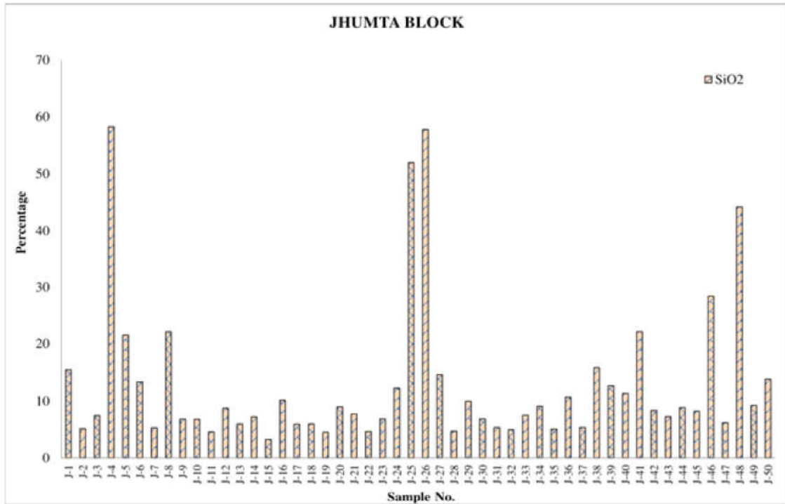
Fig. 3 : SiO 2 percentage in Limestone Samples of Jhumta
