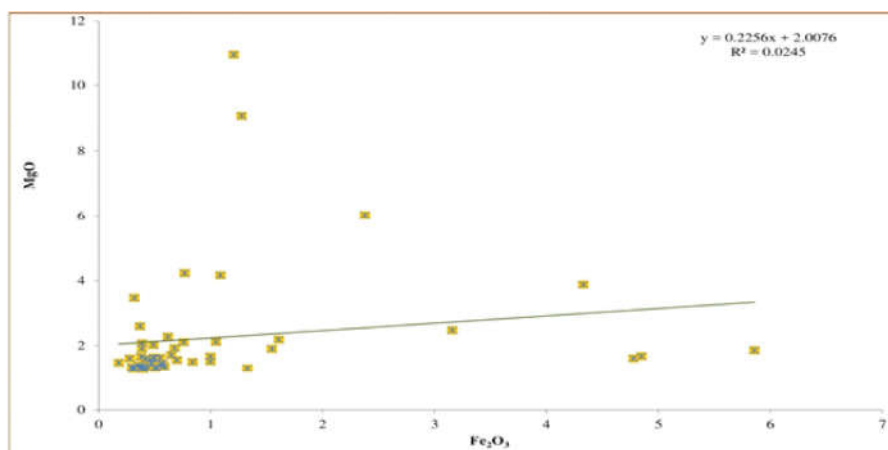
Fig. 6 : Fe 2 O 3 vs MgO percentage in Limestone Samples of Jhumta
