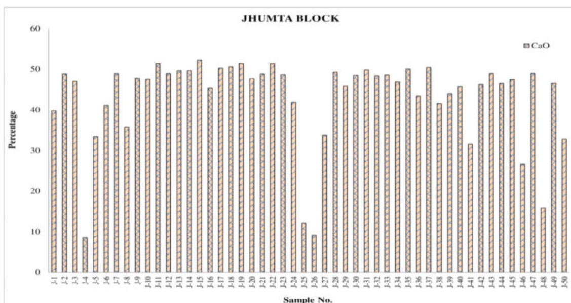
Fig. 2 : CaO percentage in Limestone Samples of Jhumta
